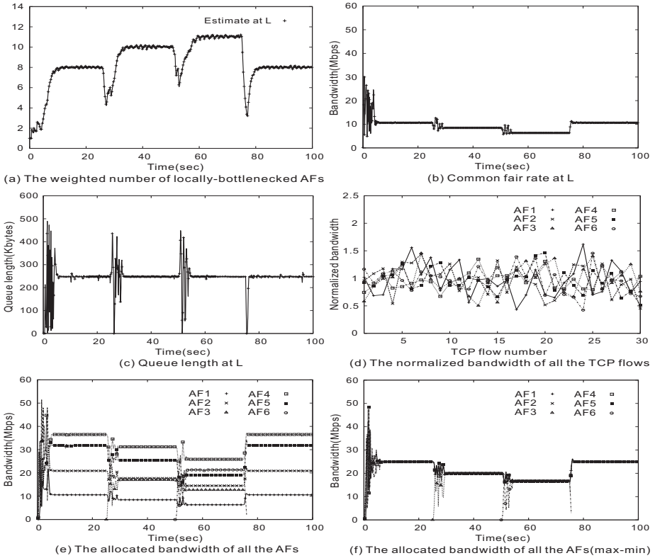
Fig. 4. Results in the single bottleneck link configuration
