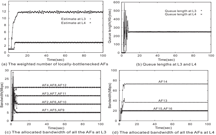
Fig. 6. Results in the multiple bottleneck link configuration
