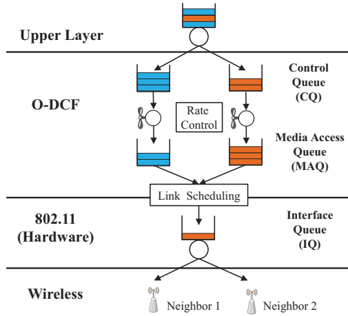
Fig. 1. Queue structure of O-DCF.
