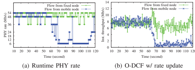
Fig. 11. Experiment. Performance evaluation in mobile scenario (Fig. 10(b)).
