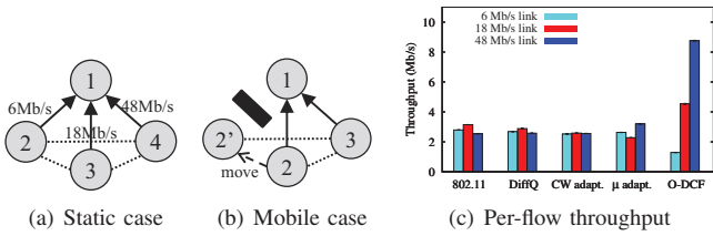
Fig. 10. Experiment. Single-hop network scenario consisting of clients and one AP; (a) static case: all nodes remain fixed with different PHY rates; (b) mobile case: node 2 moves away from node 1 at 60 seconds.
