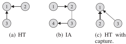
Fig. 5. Example topologies of imperfect sensing and packet capture. In network graphs, vertices represent nodes, dotted lines represent connectivity, and arrows represent flows. (a) HT; (b) IA; (c) HT with capture: a thin arrow for weak signal.
