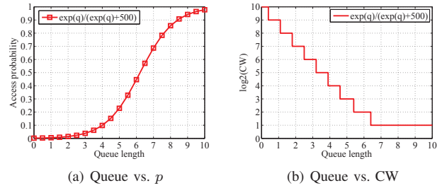
Fig. 3. Illustration of sigmoid function with respect to queue length.
