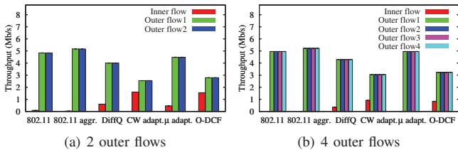
Fig. 7. FIM topology with two and four outer flows. In (a) and (b), the ideal proportional-fair throughput ratios of an outer flow and a middle flow are: 2:1 and 4:1, respectively.
