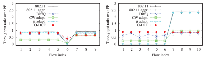
Fig. 8. Simulation. Performance comparison in two mixed topologies; the flow indexes are the same as in Fig. 4; we plot the throughput ratio over optimality: the closer to one the ratio is, the better fairness is.
